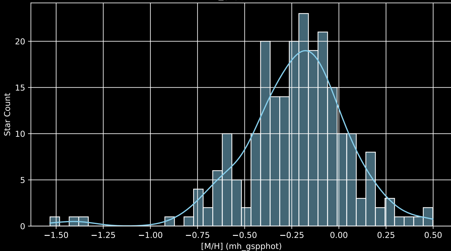
GALAH DR4 Field: [7162] [M/H] (mh_gspphot) (n= 231)
