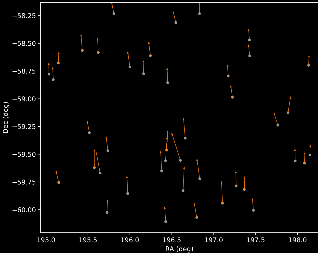
GALAH DR4 Cluster 2 Proper Motion Vectors (n=42)
