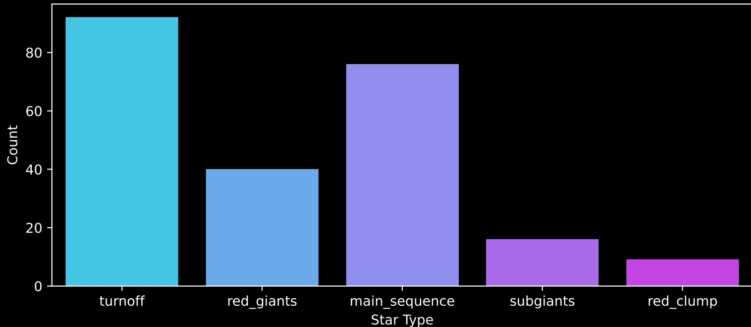
GALAH DR4 Field: [7162] Count plot of Star Type
