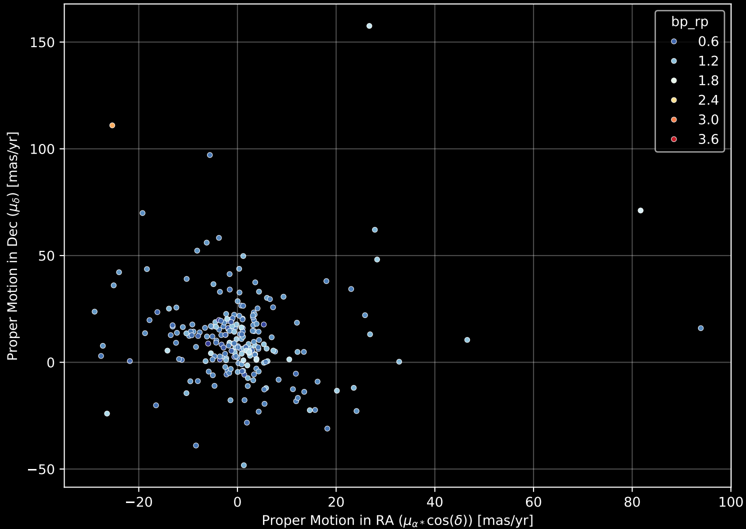
GALAH DR4 Field: [7162] Proper Motion Diagram (n= 233)
