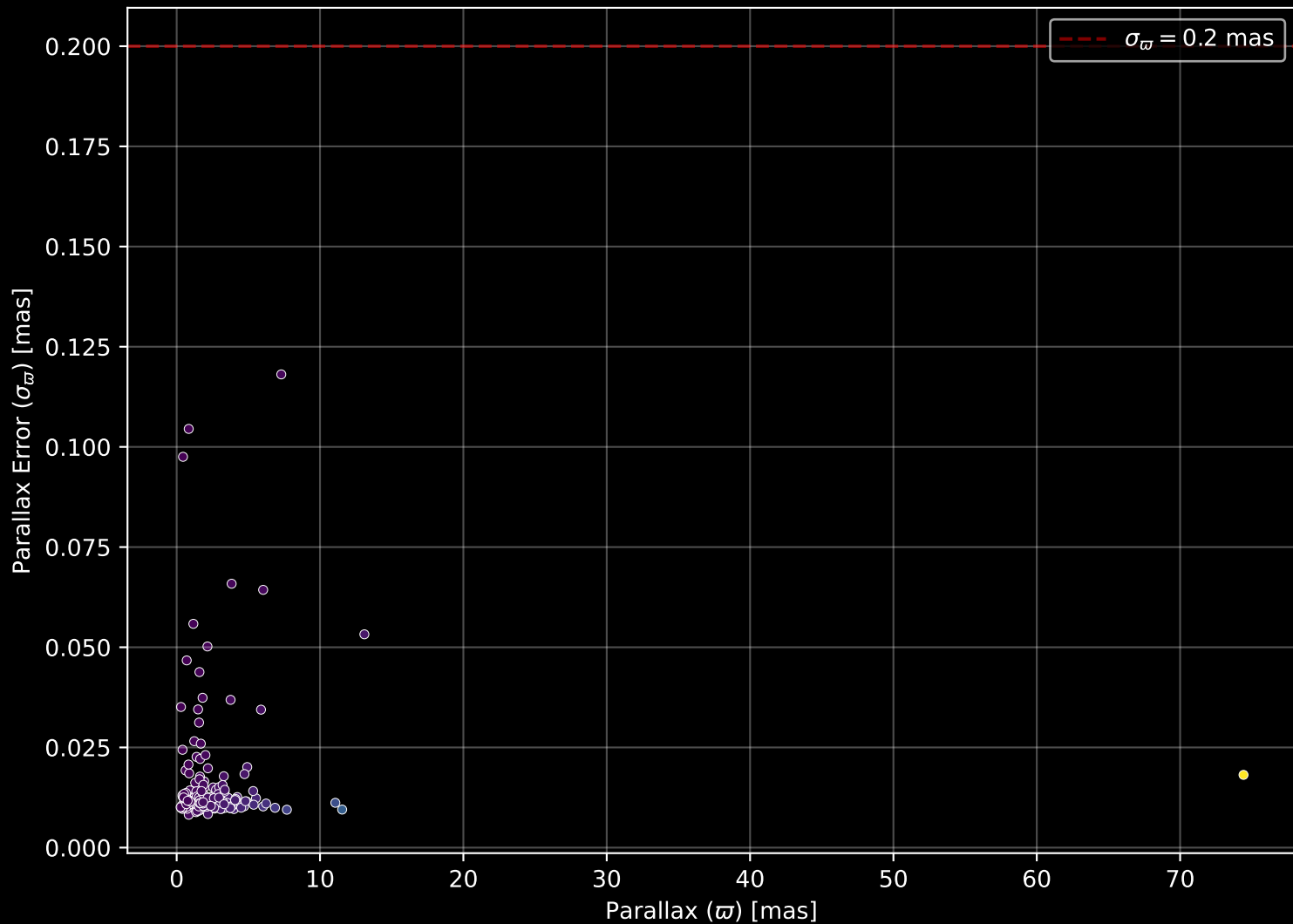
GALAH DR4 Field: [7162] Parallax Quality (n= 233)
