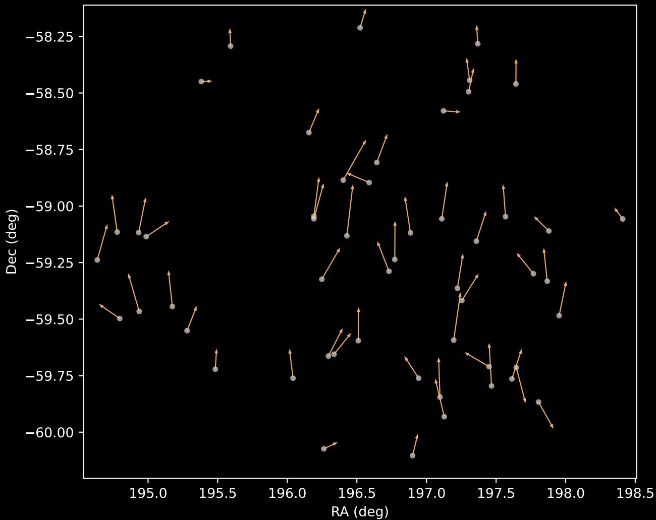
GALAH DR4 Cluster 3 Proper Motion Vectors (n=53)
