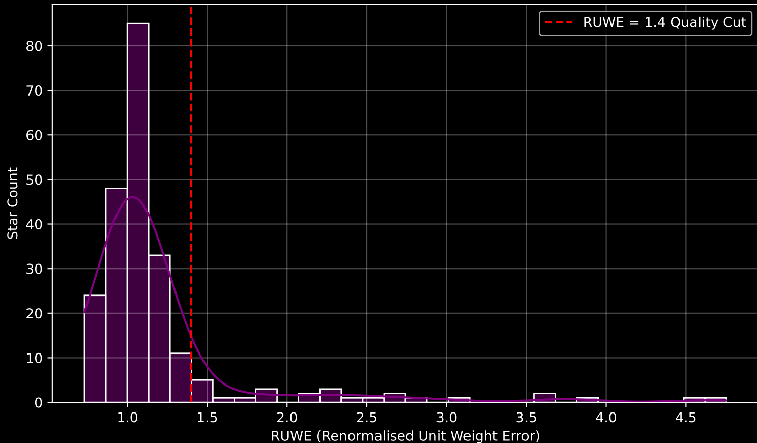
GALAH DR4 Field [7162] RUWE Distribution (n= 227)
